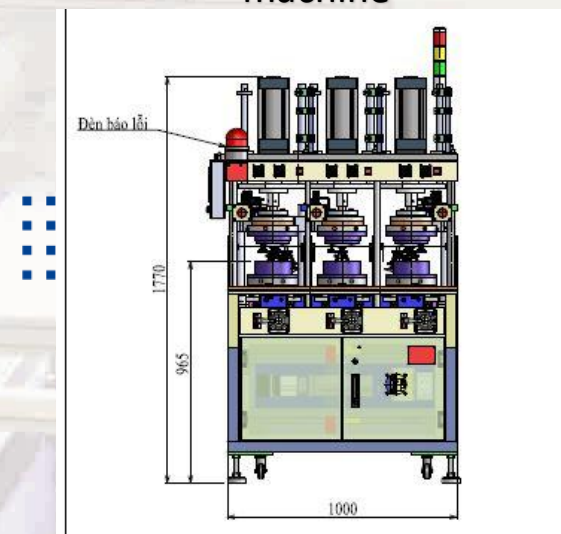
Heat and stamping machine
